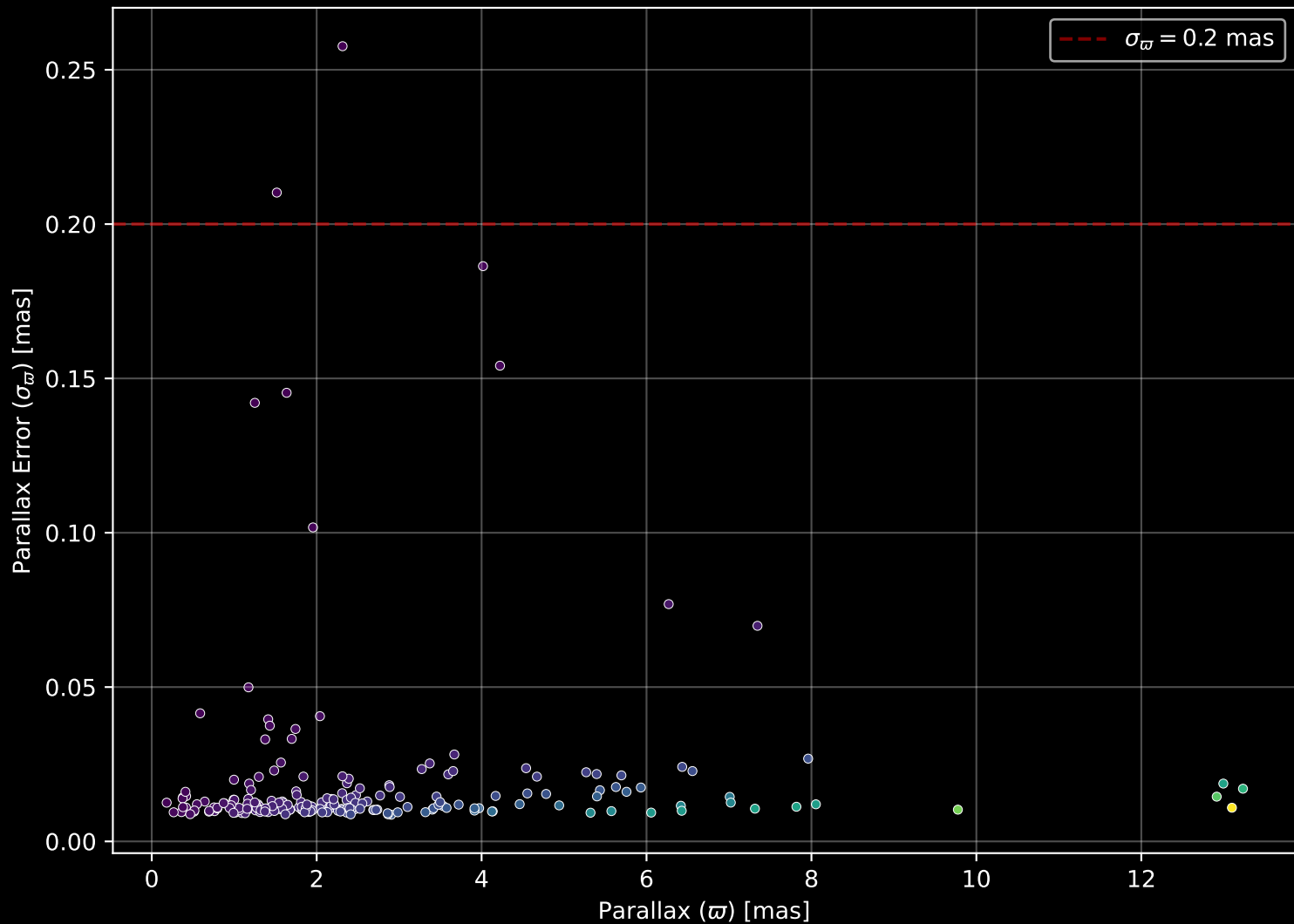
APOGEE DR17 Field: [251-33] Parallax Quality (n= 214)
