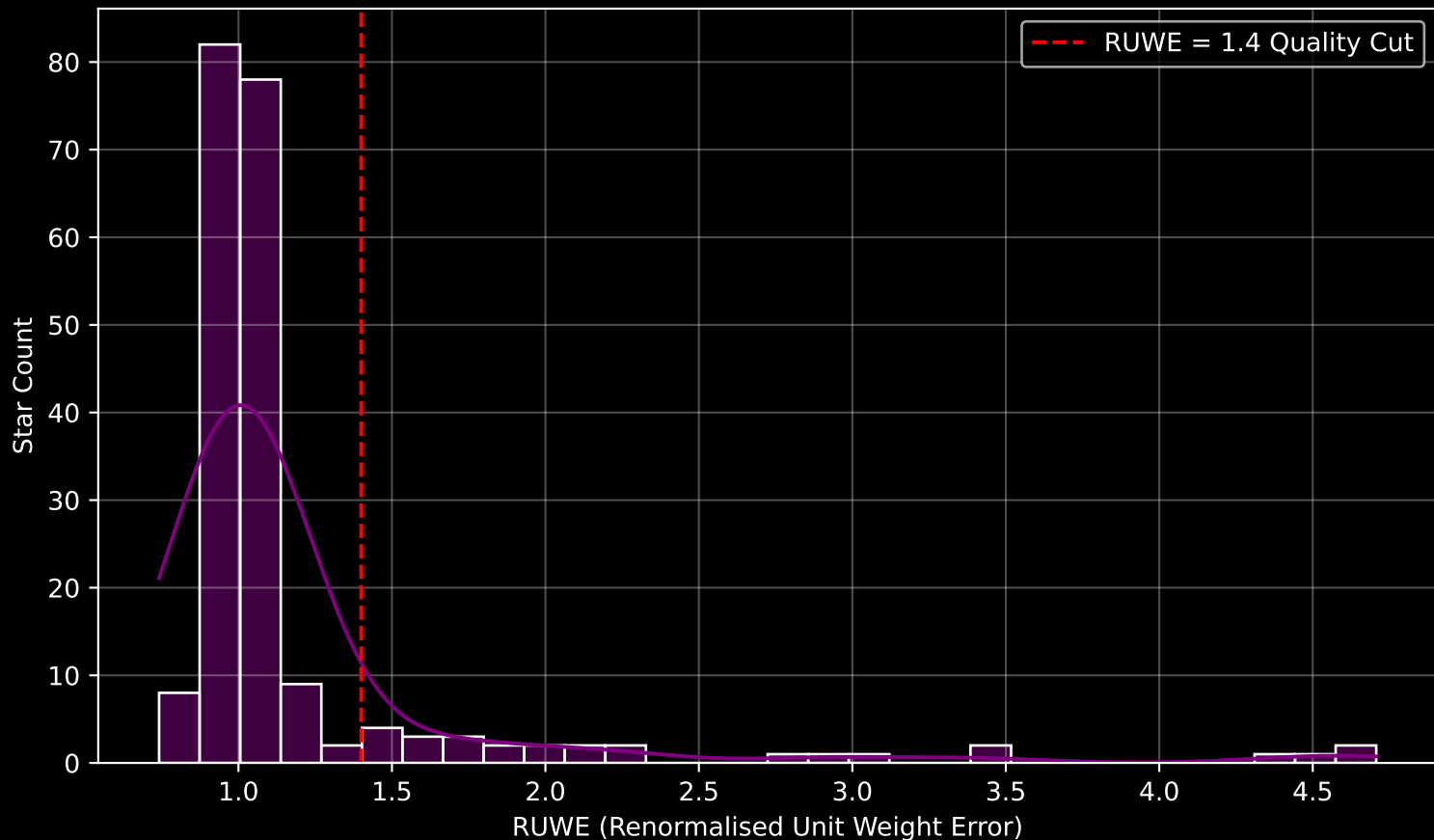
GAPOGEE DR17 Field [251-33] RUWE Distribution (n= 206)
