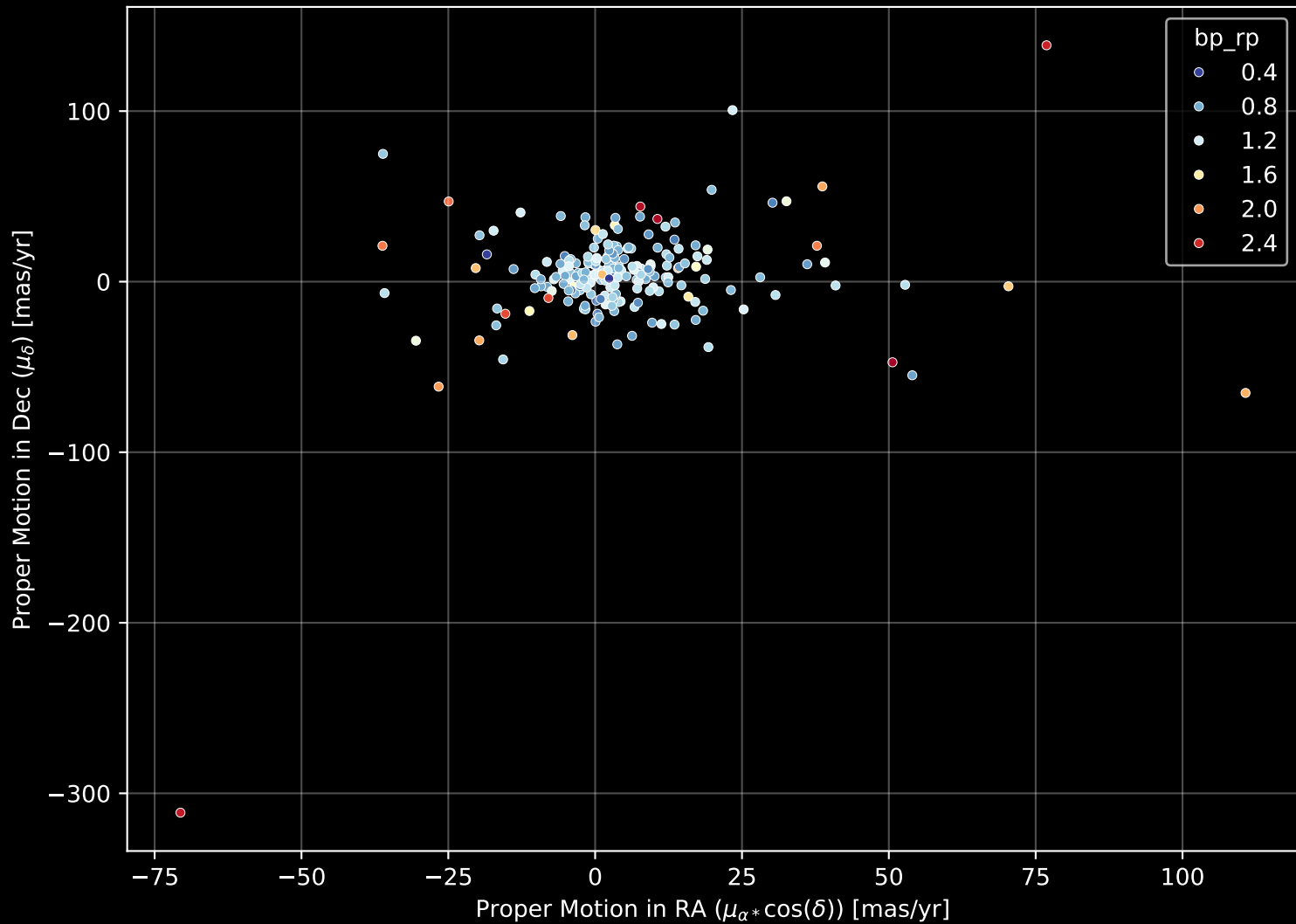
APOGEE DR17 Field: [251-33] Proper Motion Diagram (n= 214)
