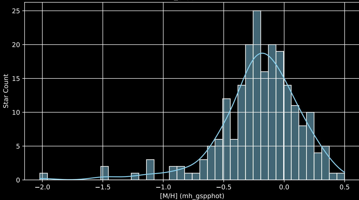
APOGEE DR17 Field: [251-33 [M/H] (mh_gspphot) (n= 213)
