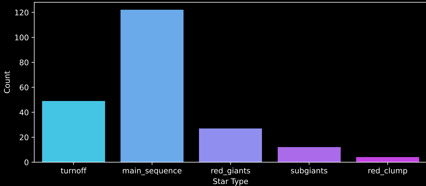
APOGEE DR17 Field: [251-33] Count plot of Star Type
