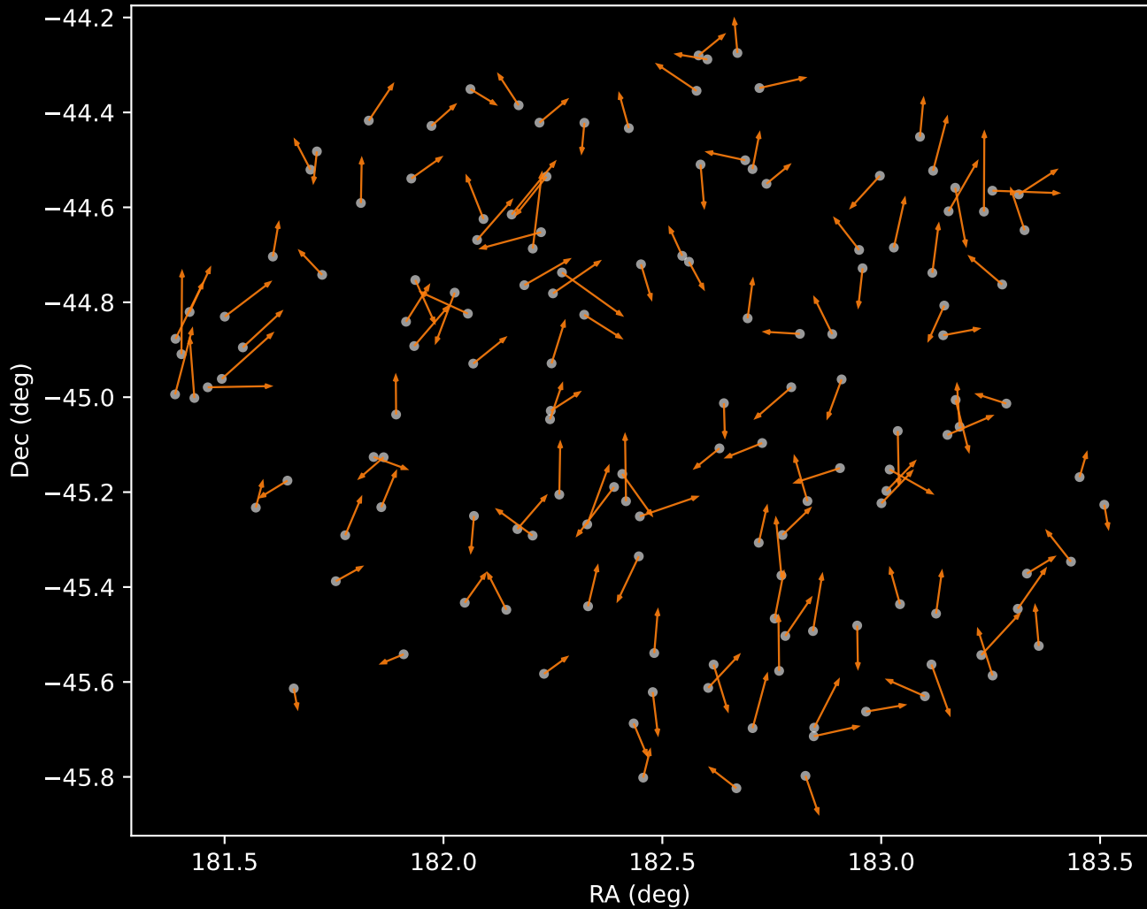
APOGEE DR17 Cluster 2 Proper Motion Vectors (n=143)
